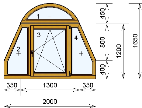
Pos. 17, 1 St.
